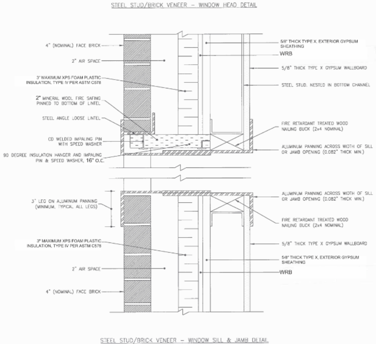
FIGURE 1 WINDOW AND DOOR OPENING DETAILS
