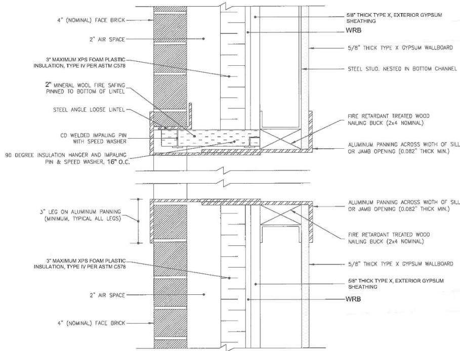
STEEL STUD/BRICK VENEER - WINDOW SILL & JAMB DETAIL
